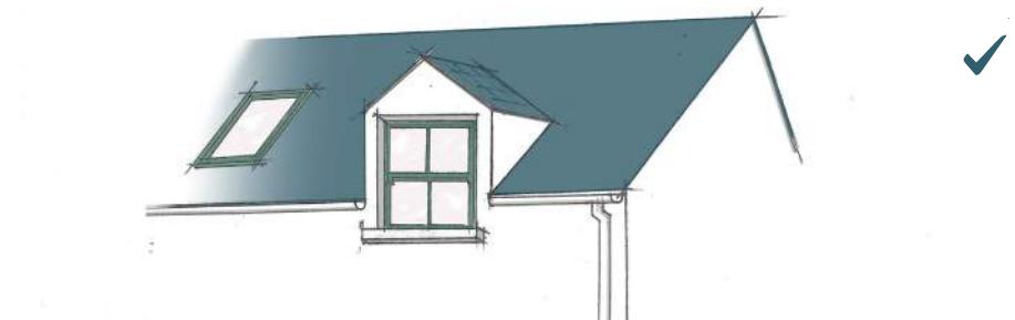
Simple eaves with dormer window extended out of the facade in matching render. Symmetrical rooflights recommended to reduced building scale.
